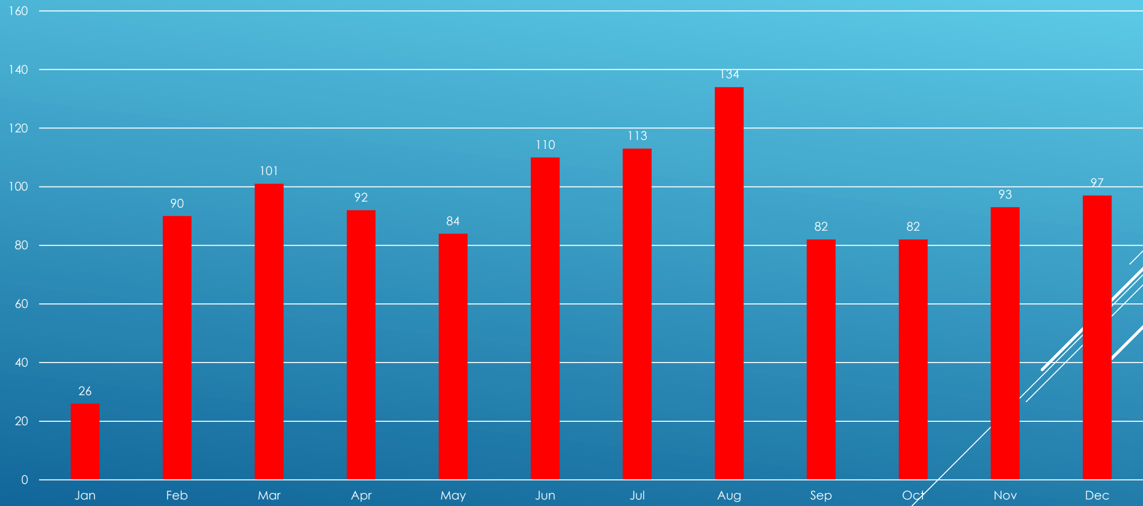
Ionia Dept. Public Safety Monthly CFS - Fire
