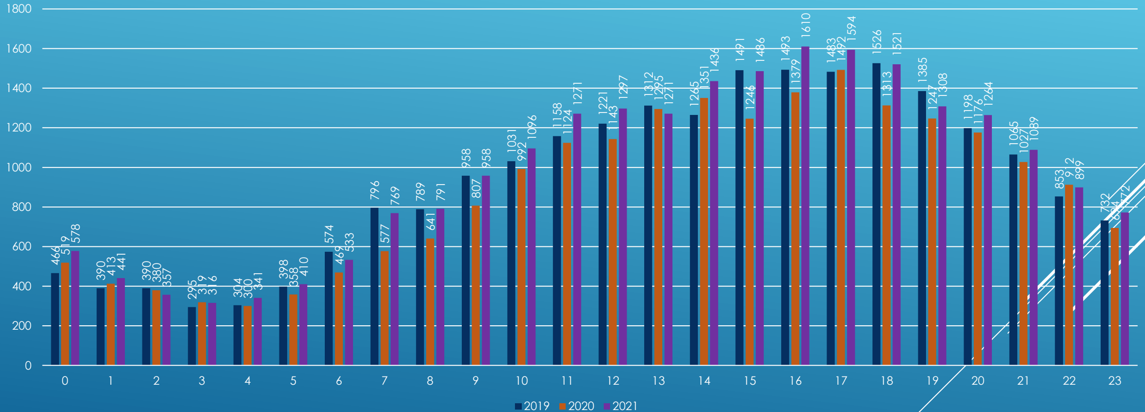
911 CALLS BY HOUR OF DAY
