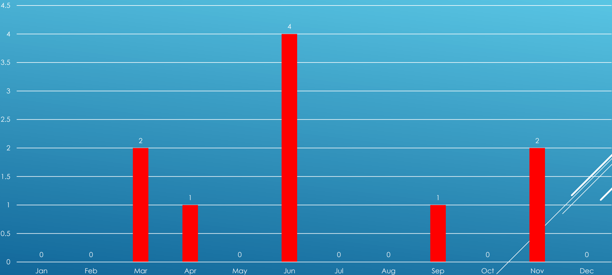
Freeport Fire CFS by Month
