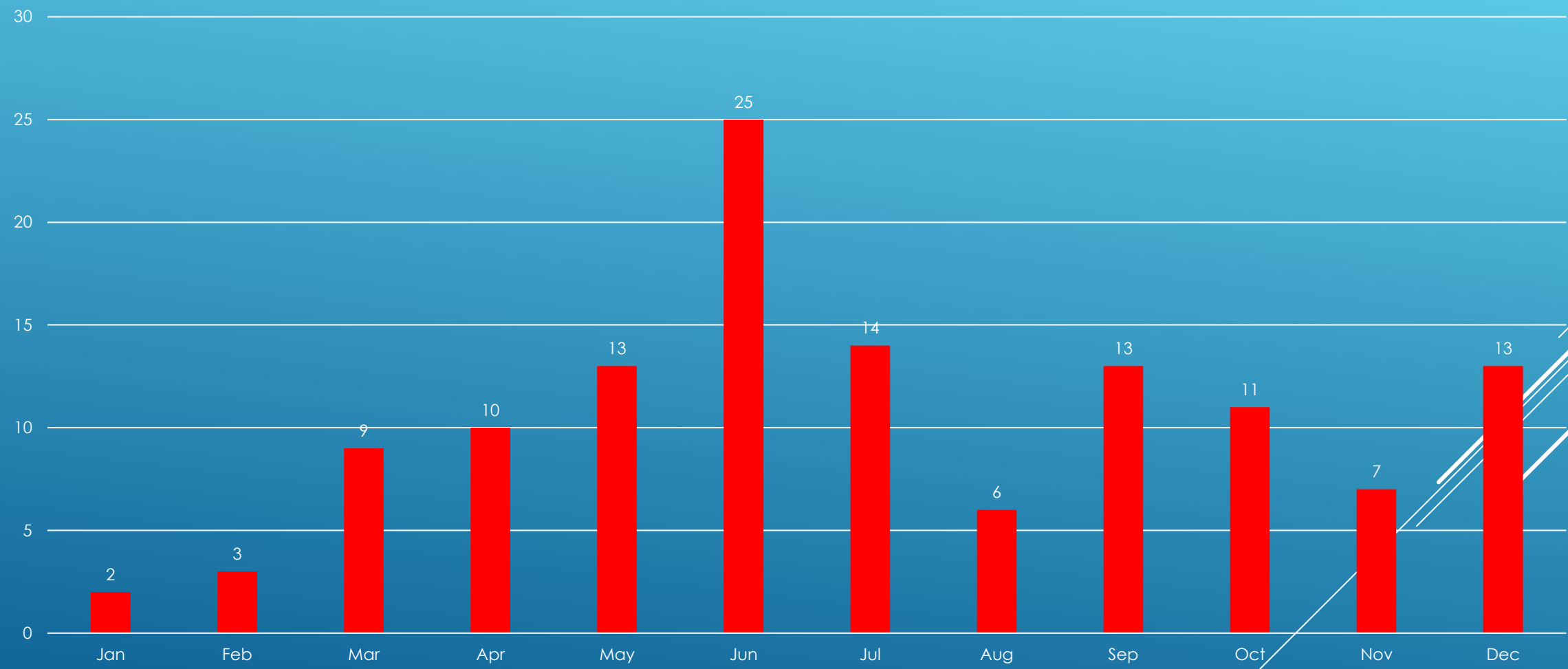
PEWAMO FIRE MONTHLY CFS
