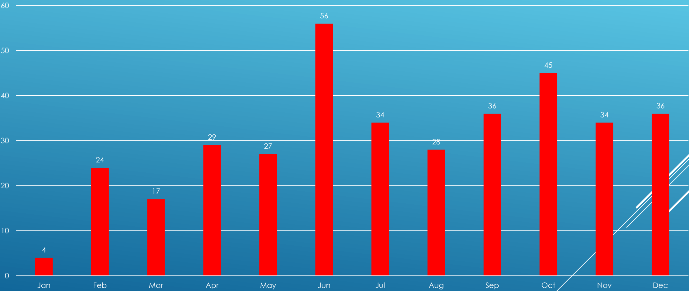
Lake Odessa Fire Dept. Monthly CFS
