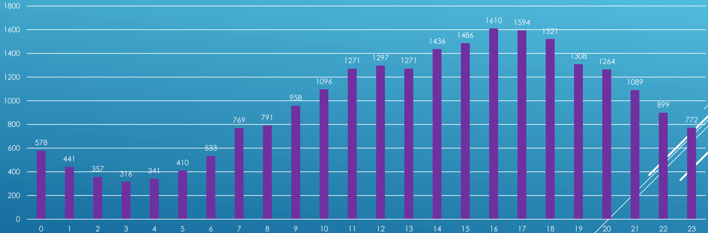
911 Calls by Hour of Day 2021
