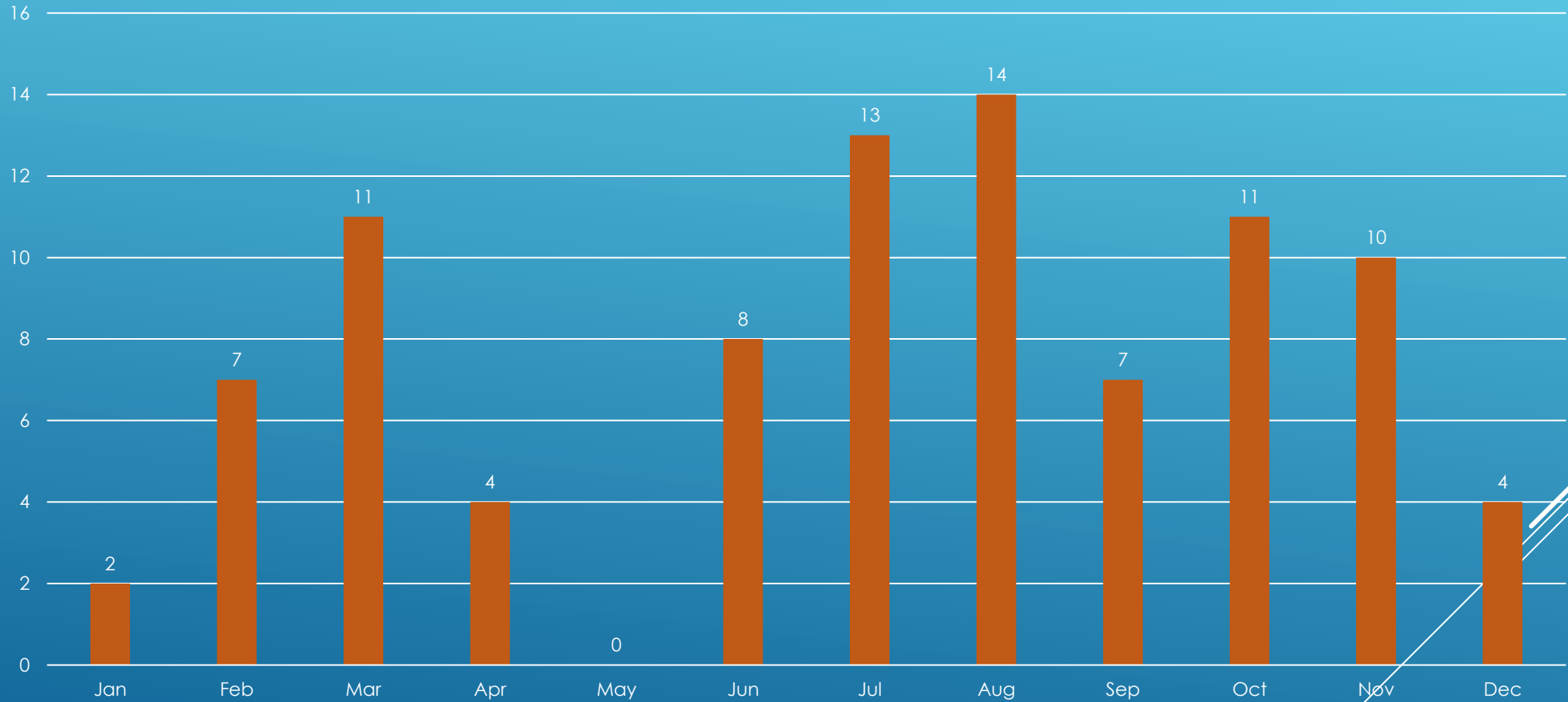
Animal Control Monthly CFS
