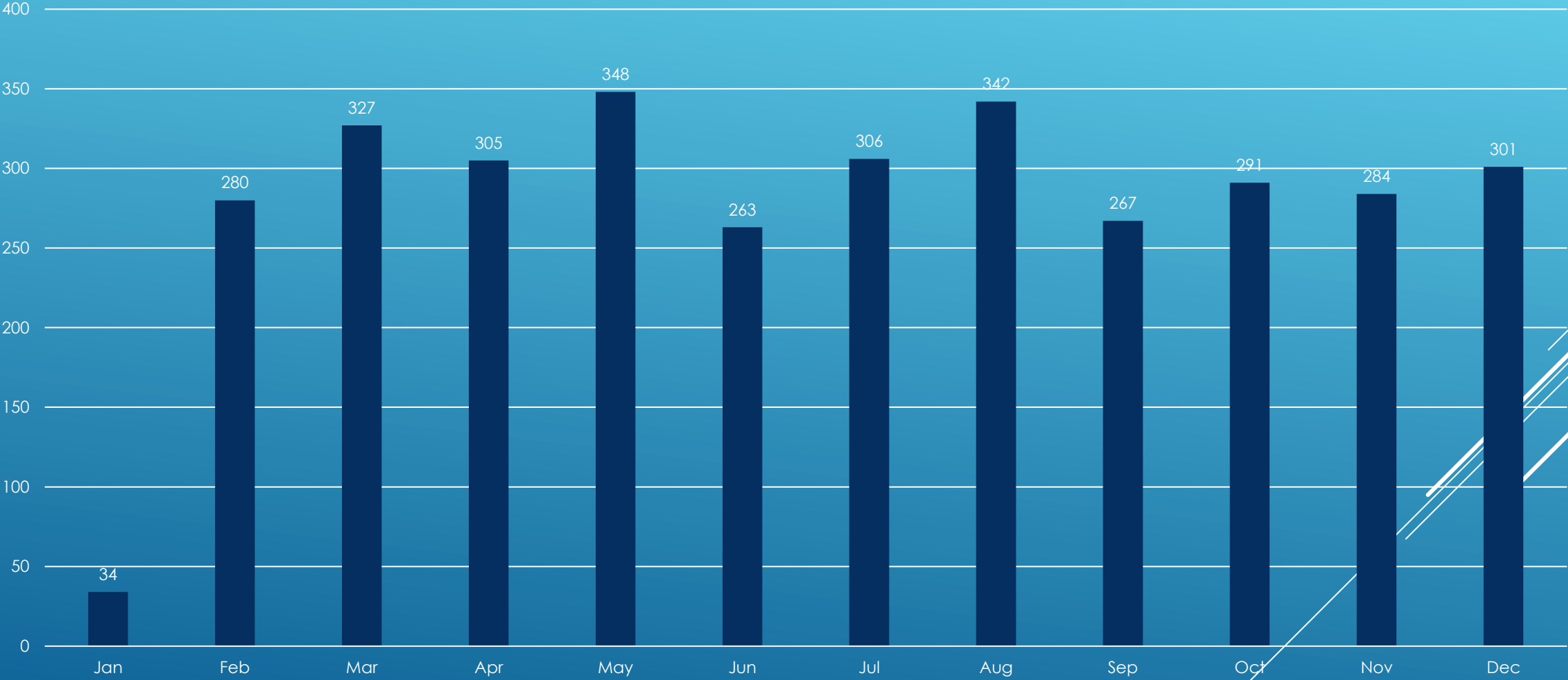
Belding CFS Monthly
