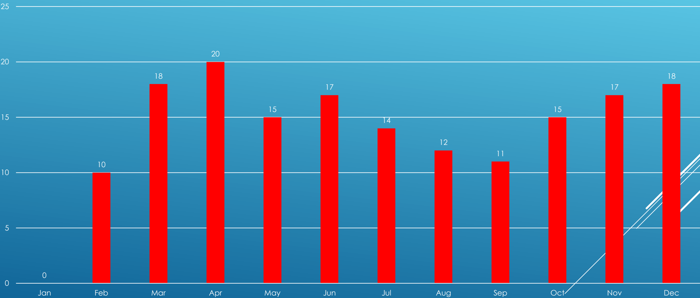
Clarksville Fire Monthly CFS
