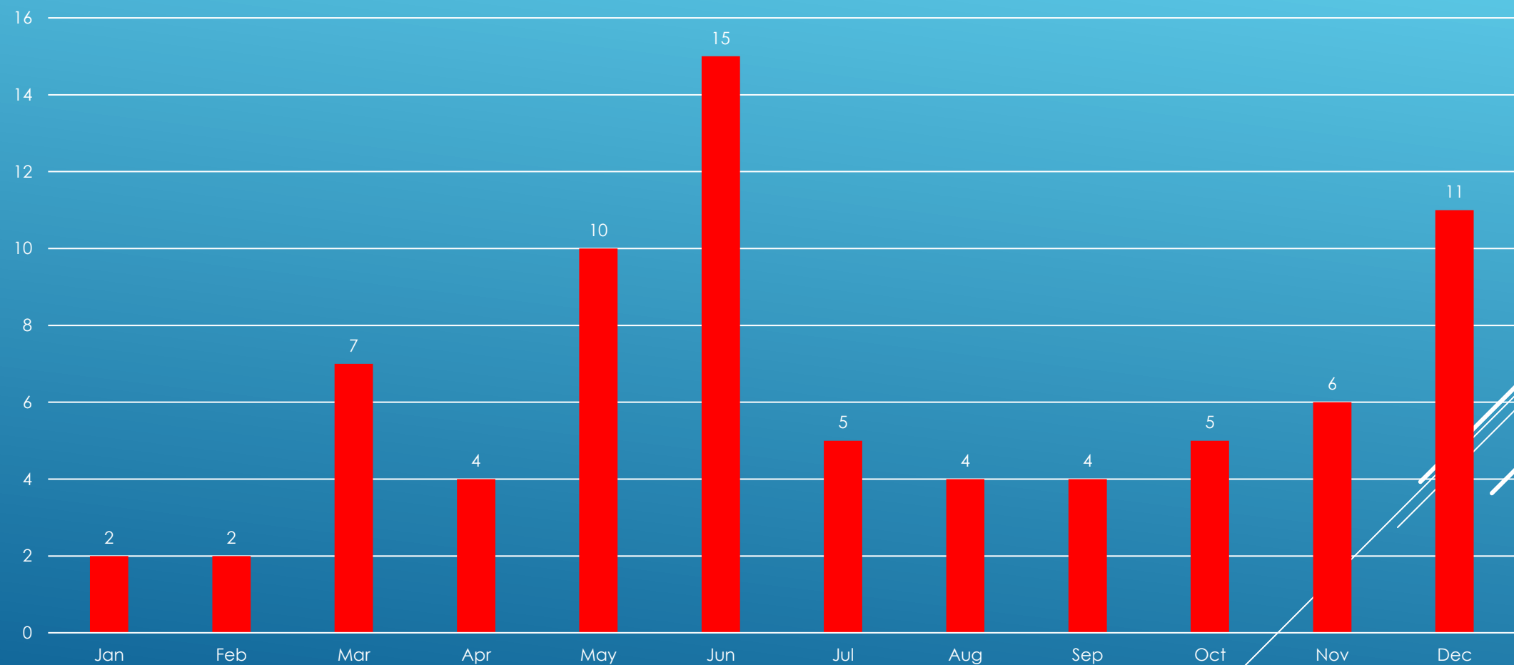
Hubbardston Fire Monthly CFS
