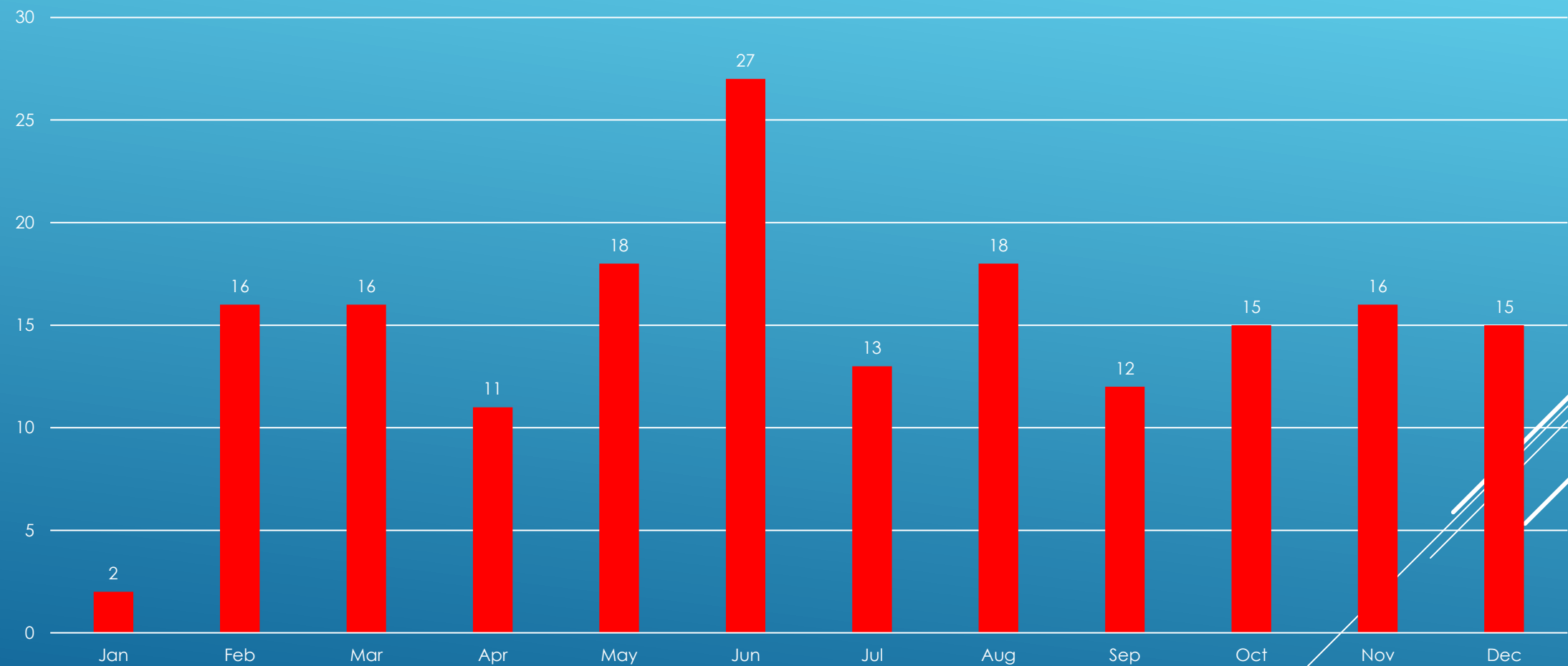
Ronald Fire Monthly CFS
