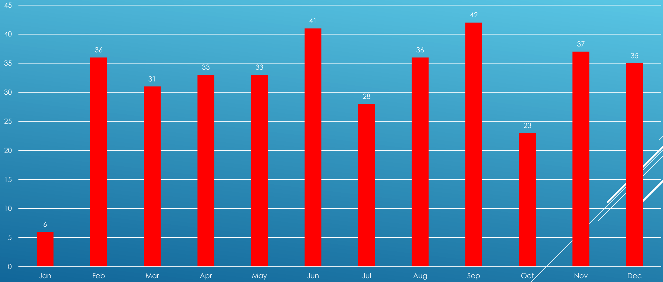
Berlin-Orange FD Monthly CFS
