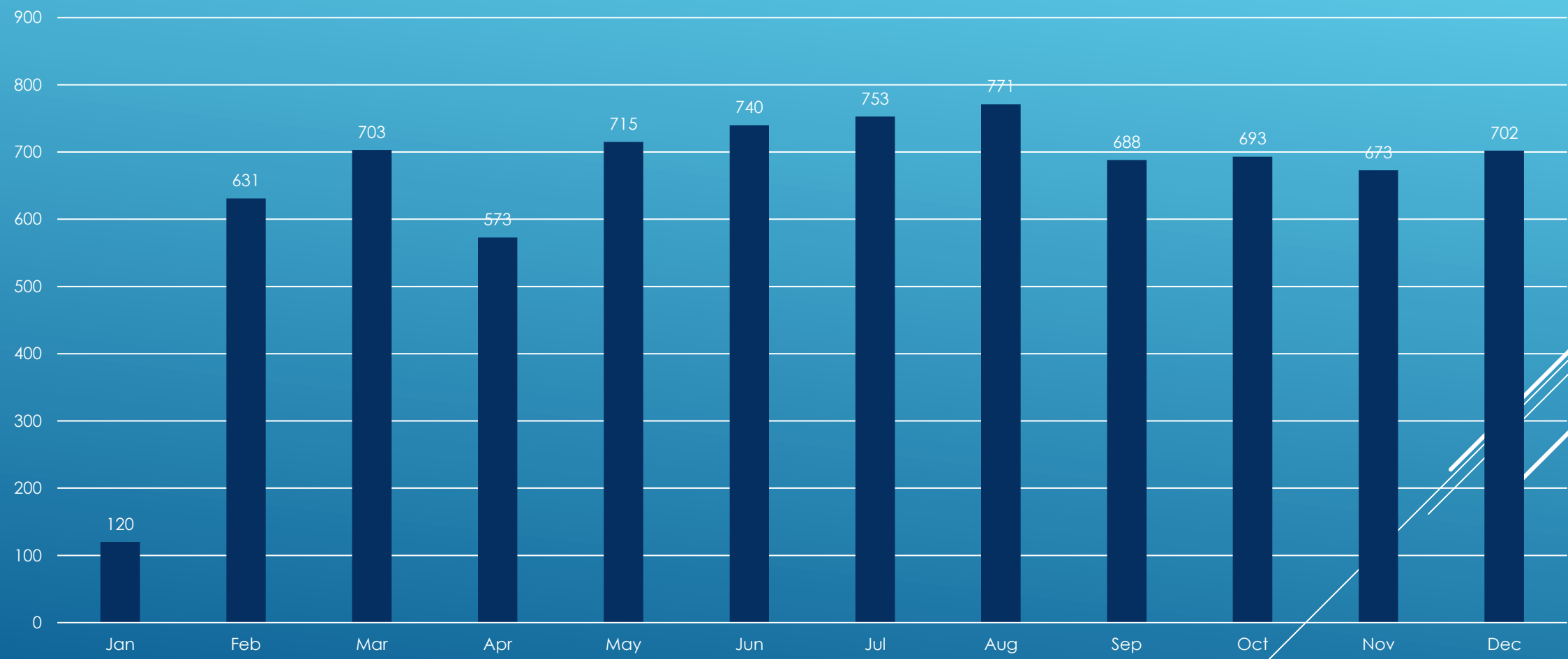
ICSO Monthly CFS - Total 7762
