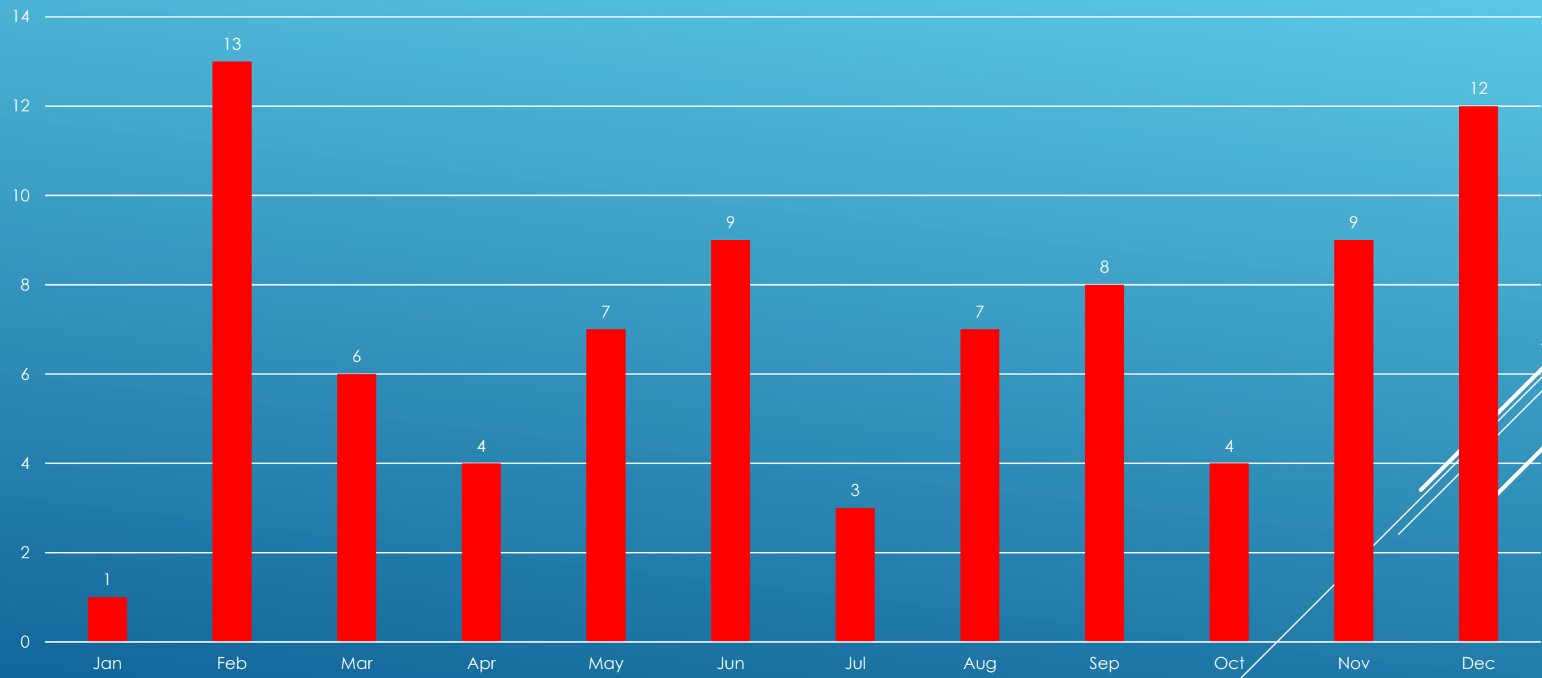
Sunfield Fire Monthly CFS
