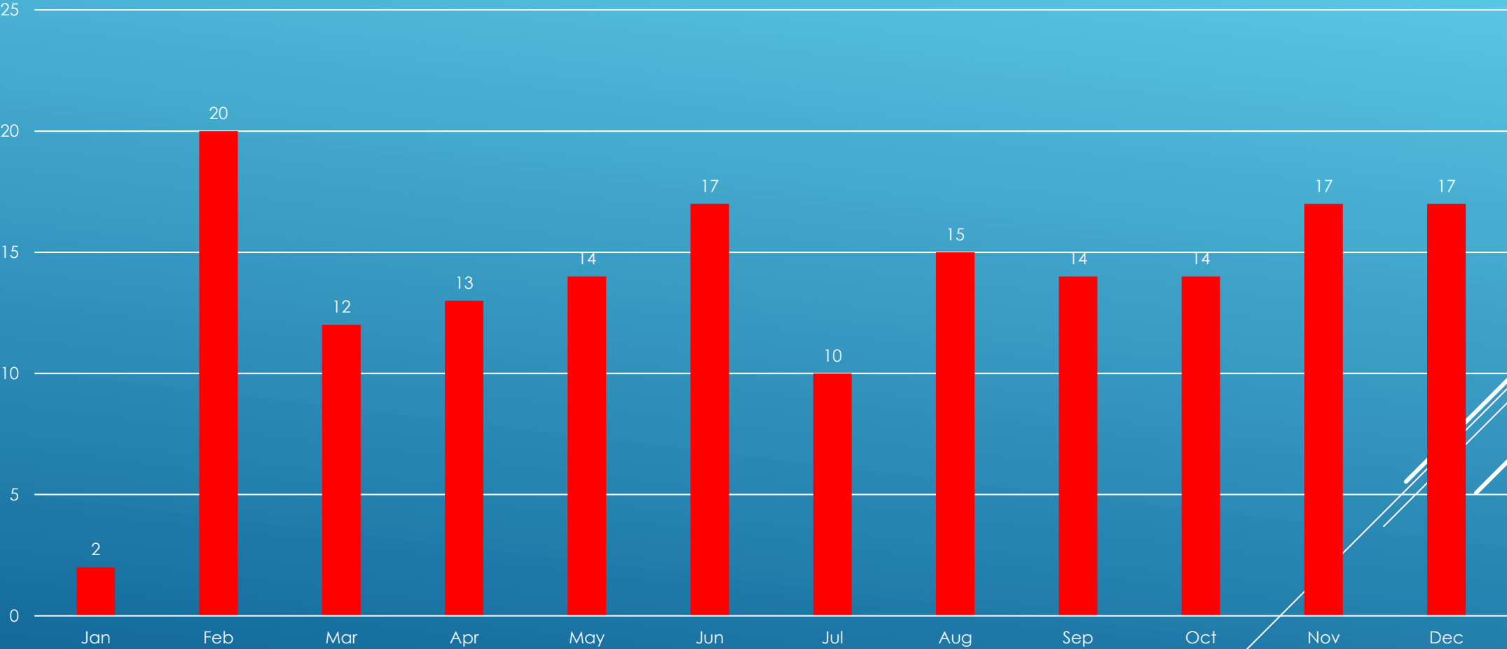
Portland Fire Monthly CFS
