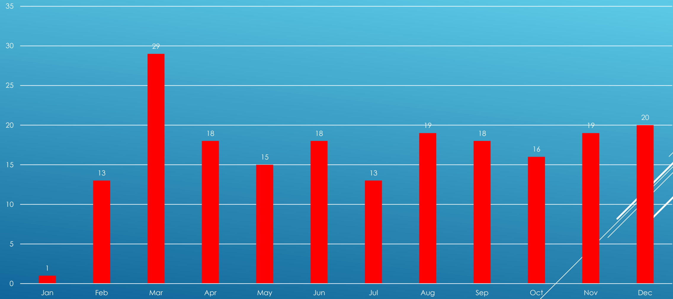
ORLEANS FIRE MONTHLY CFS
