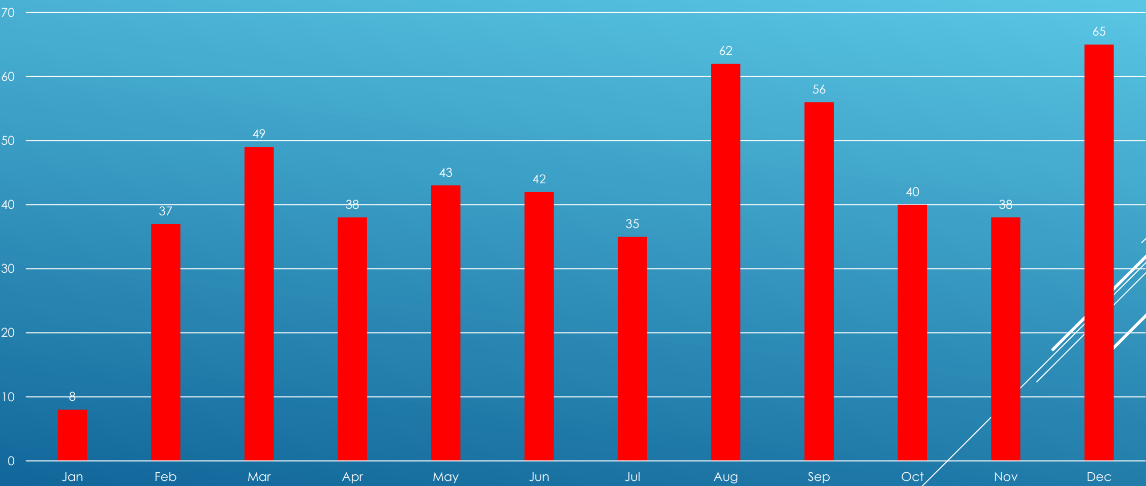
Saranac Fire Monthly CFS
