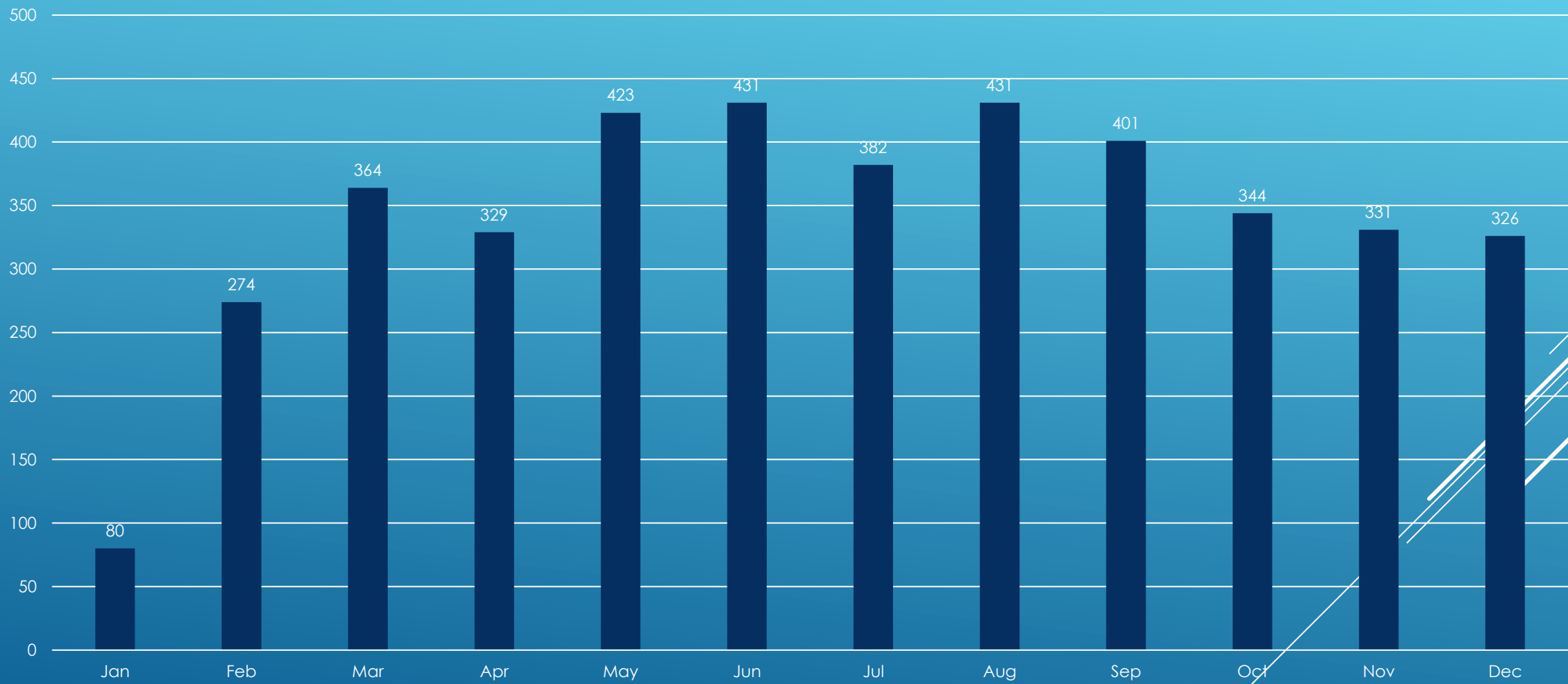
Ionia Dept. Public Safety Monthly CFS - Law
