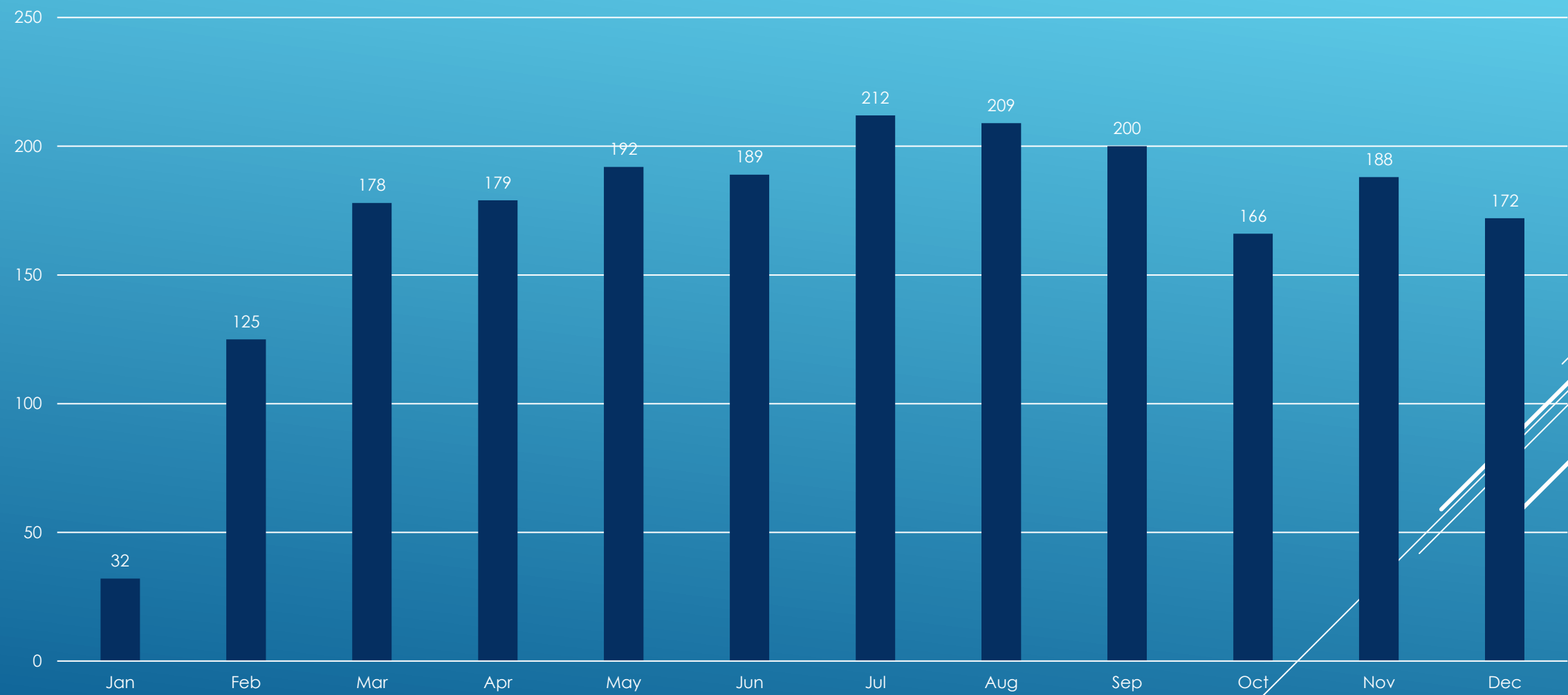
Portland Police Monthly CFS
