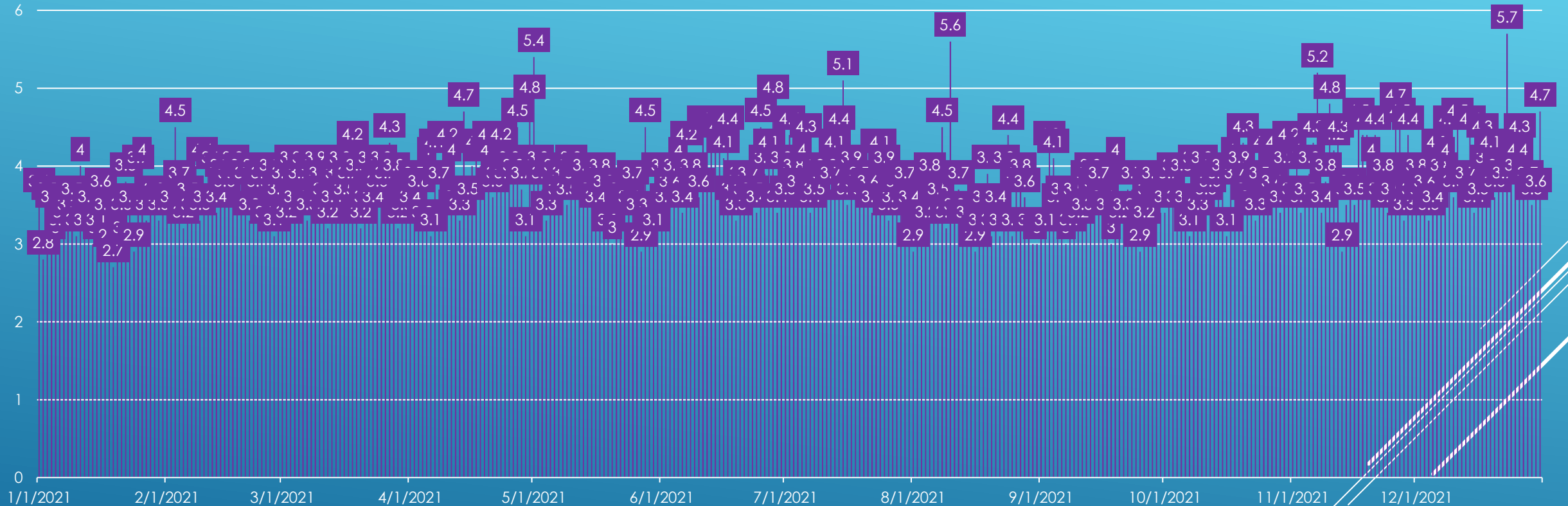
2021 DAILY AVERAGE 911 CALL RING TIME
