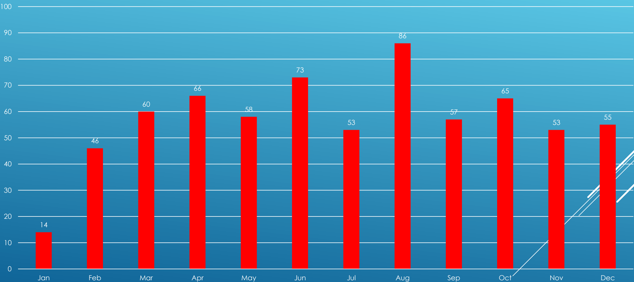
Belding Fire Department CFS Monthly
