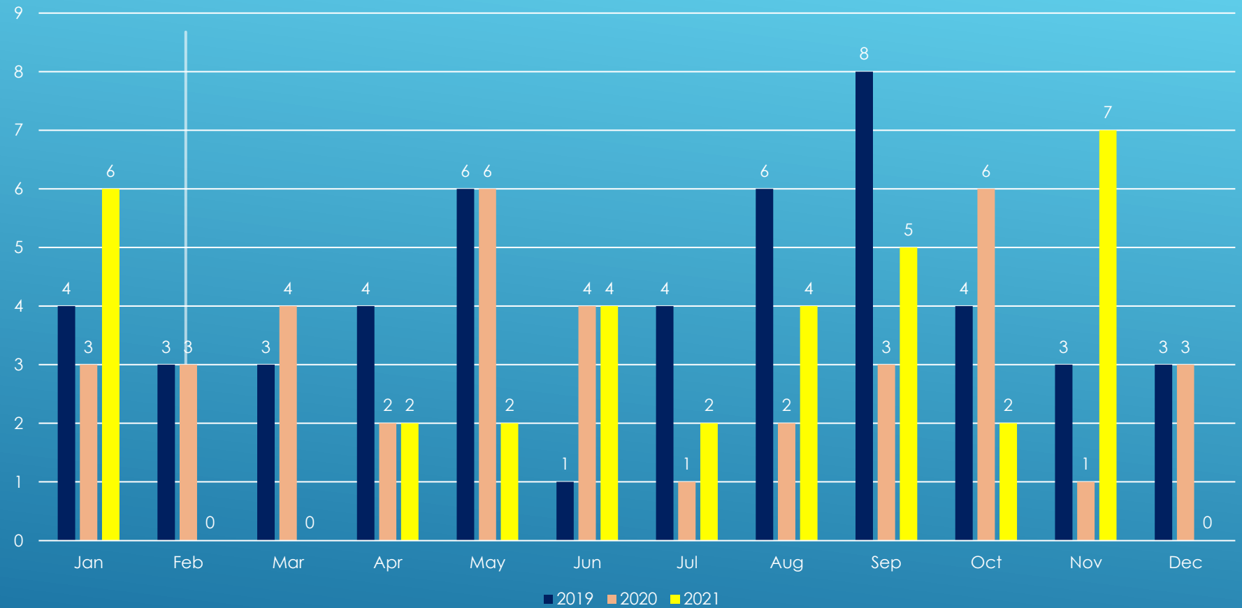
Text to 911 Monthly Text Contacts
