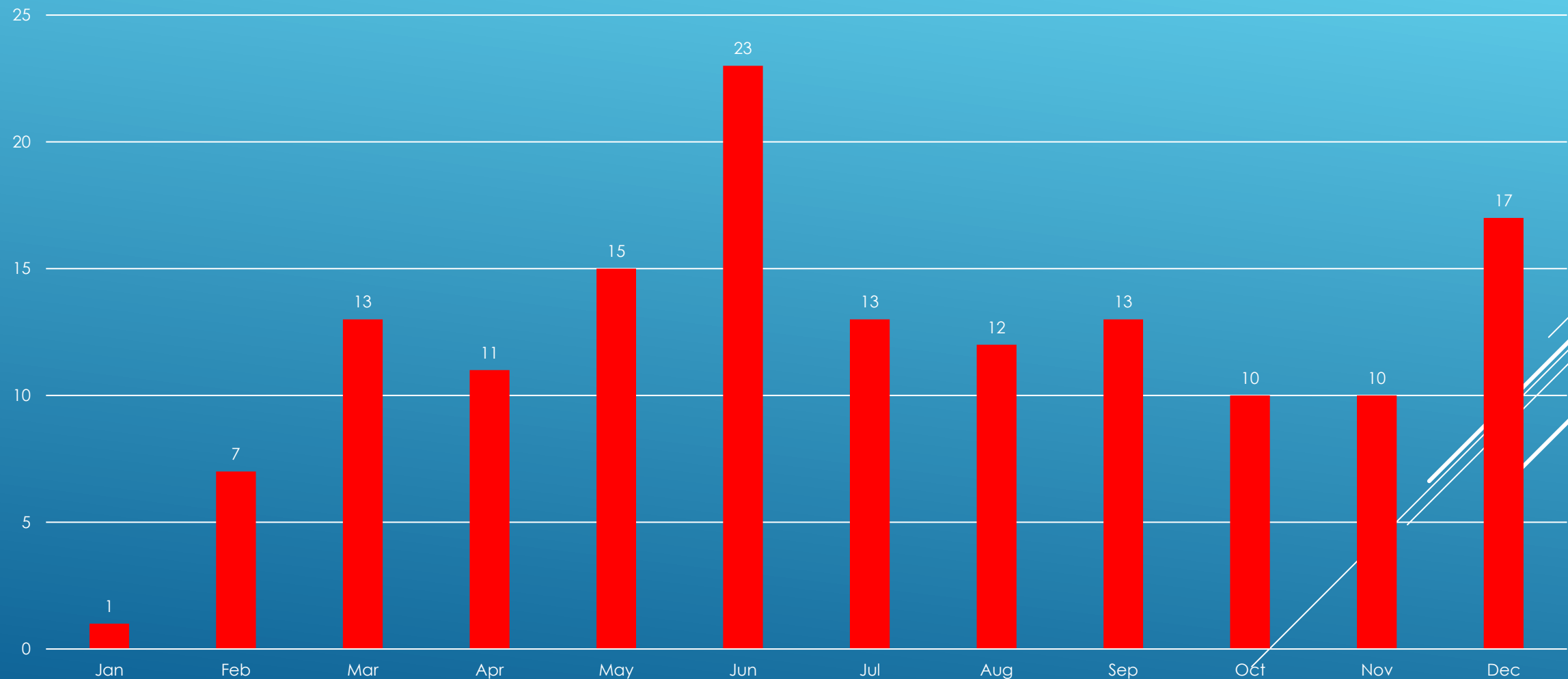
LYONS-MUIR FIRE DEPT. MONTHLY CFS
