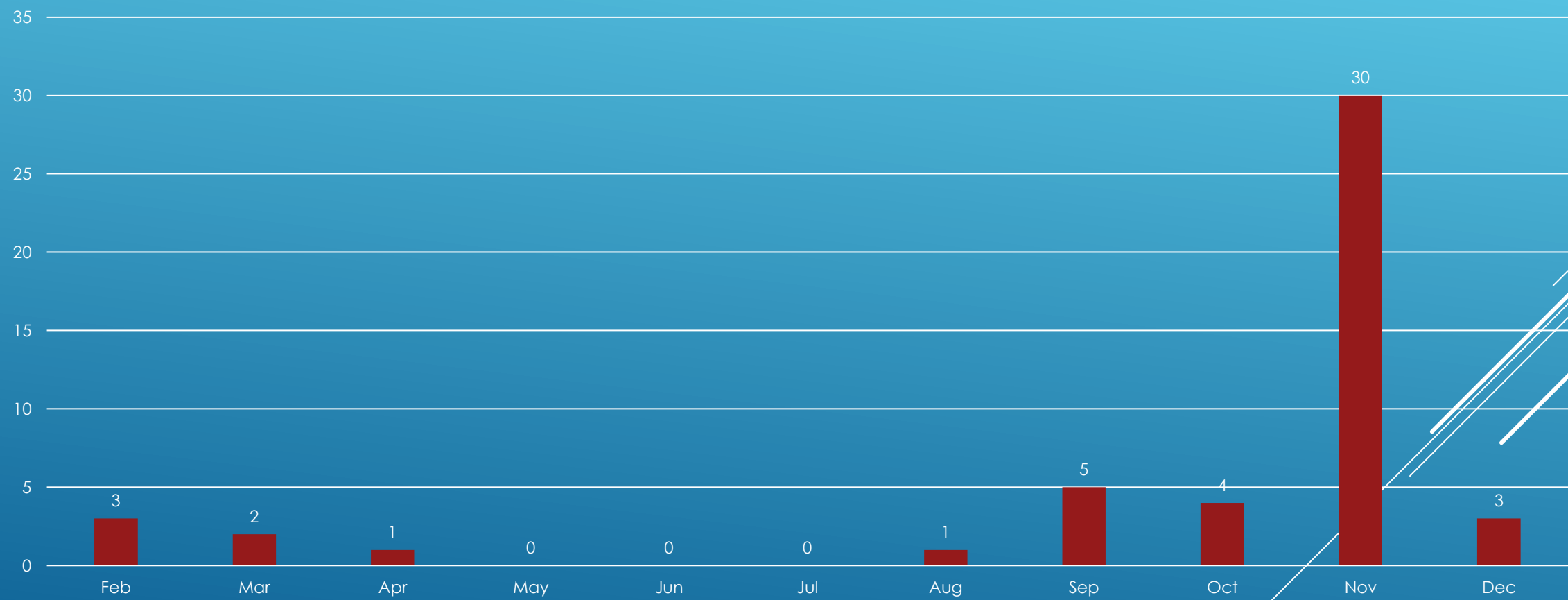
DNR MONTHLY CFS
